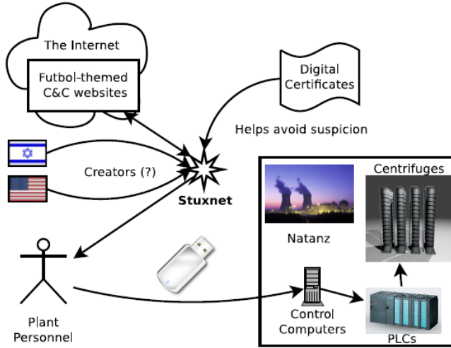
Figure 1: A high-level overview of Stuxnet.
